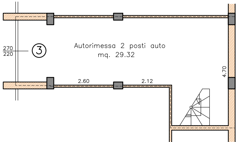
PIANO TERRA
